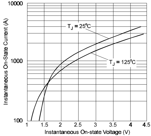
Fig. 11 - On-state Voltage Drop Characteristics
