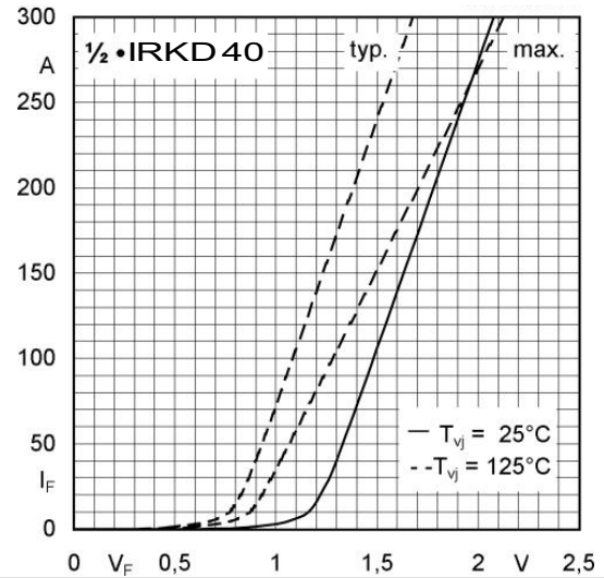
Fig. 15 Forward characteristics
