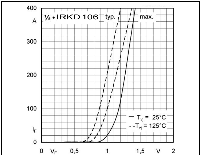
Fig. 15 Forward characteristics
